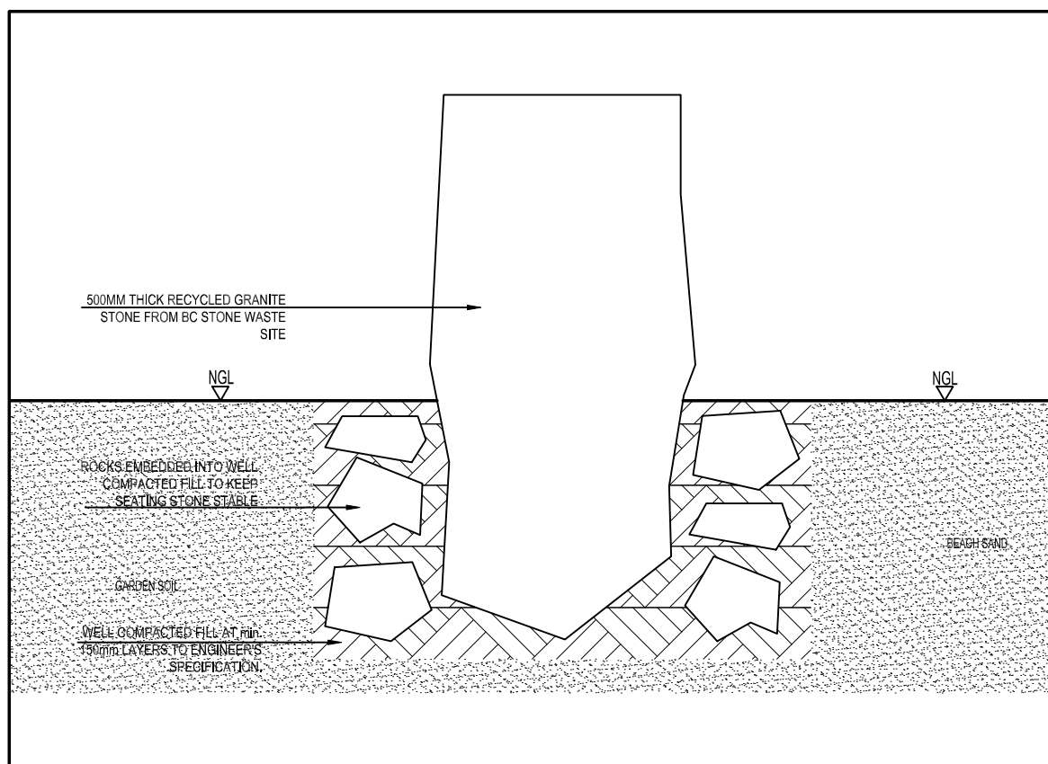
SECTION - A 1:25
