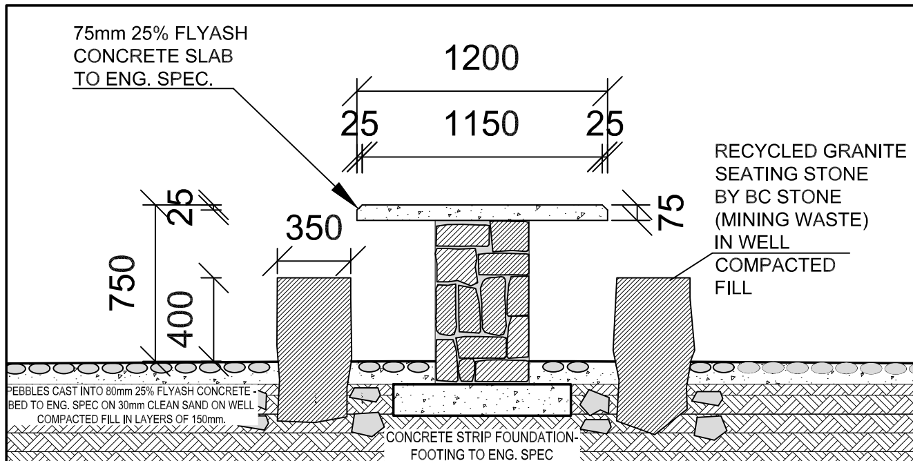
SECTION - A 1:25
